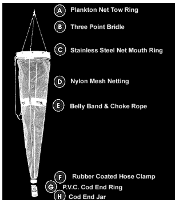
Plankton Net components
