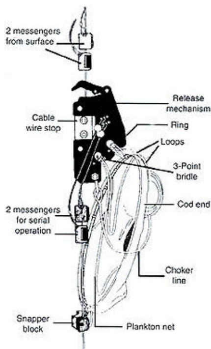
Typical Double-Release Mechanism Loading
