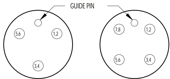
CONTACT CONFIGURATIONS (IEB6/8M FACE VIEWS)
