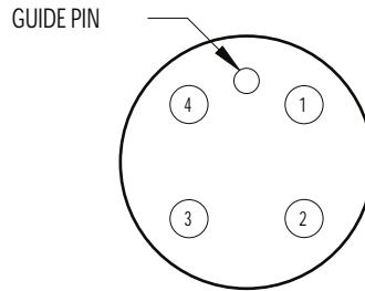
CONTACT CONFIGURATIONS (IEB34M FACE VIEW)
