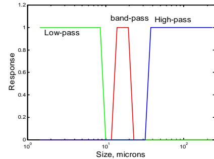
Figure 4: The LISST-25X embodies specially shaped focal-plane detectors that can permit the user to select the size-range over which TSS is to be measured. As example, a user may choose to ignore the wash-load in a stream, or use the LISST-25X to measure the wash-load only.
