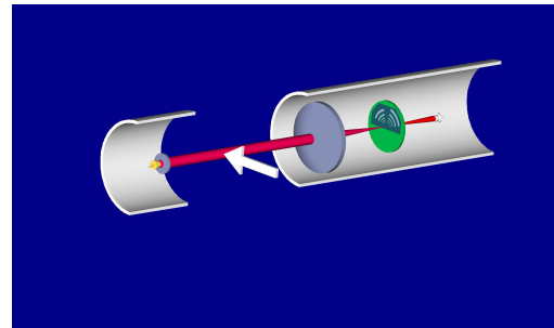
Figure 2: This is the LISST-100 . A collimated laser beam emanates from left. Particles in the flow scatter light. A receiving lens collects the scattered light, which is detected by the ring detector . A hole in the center of the ring detector permits the focused laser beam to pass through, where its power is sensed. This constitutes a transmission measurement. This measurement corrects for attenuation of the scattered light that is sensed by the rings.
