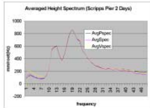
Figure 2. 1200 kHz ADCP deployed off Scripps Pier in 12 meters depth. Upper frequency is band 0.35 Hz.
