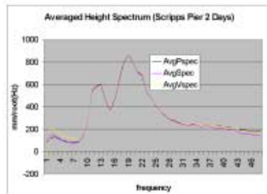
Figure 2. 1200 kHz ADCP deployed off Scripps Pier. CA- in 12 meters depth. Upper frequency is band 0.35 Hz.
