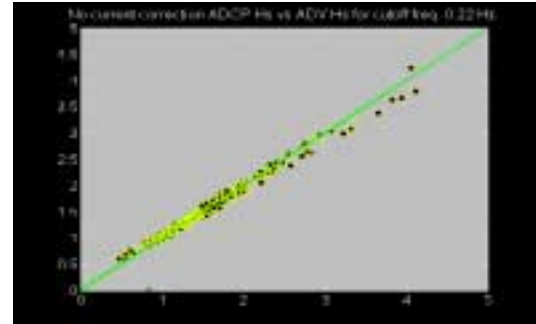
Figure 13. . Scatter plot showing that by neglecting currents, the ADCP and reference H_s measurements match.
