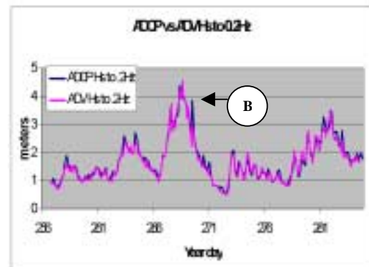
Figure 10. Differences between ADCP H_s and reference data remain even with identical cut-off frequency.
