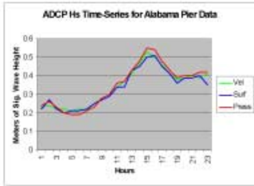
Figure 3. 1200 kHz ADCP data collected from a pier in Gulf Shores, AL in 3 meters water depth.
