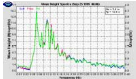
Figure 1. Wave amplitude spectra ( m/\sqrt{Hz} ) derived from pressure, ADCP velocity, and surface track measurements. Data are from Grays Harbor, WA.
