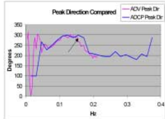
Figure 16. Peak directions for PUV and ADCP wave measurements at Grays Harbor.
